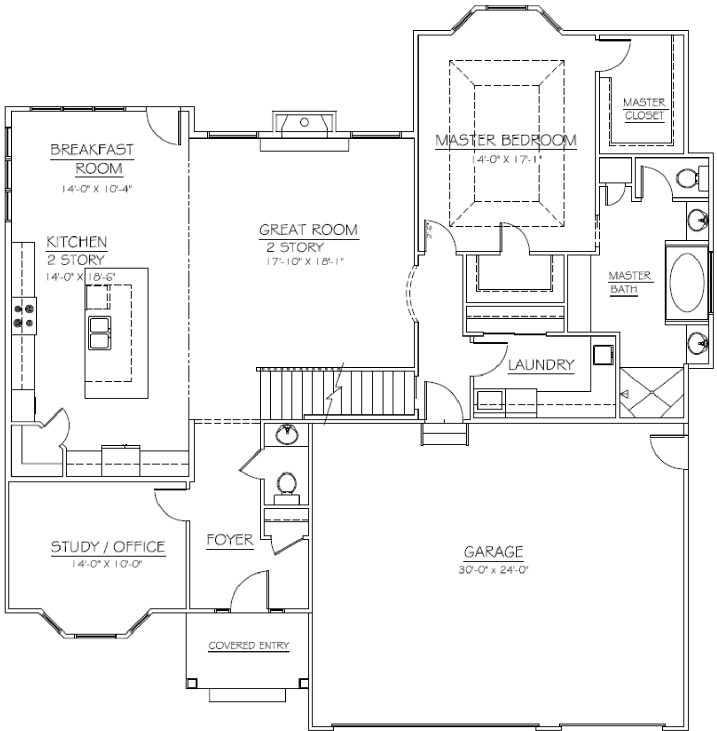
First Floor Plan 1,871 Sq. Ft.
