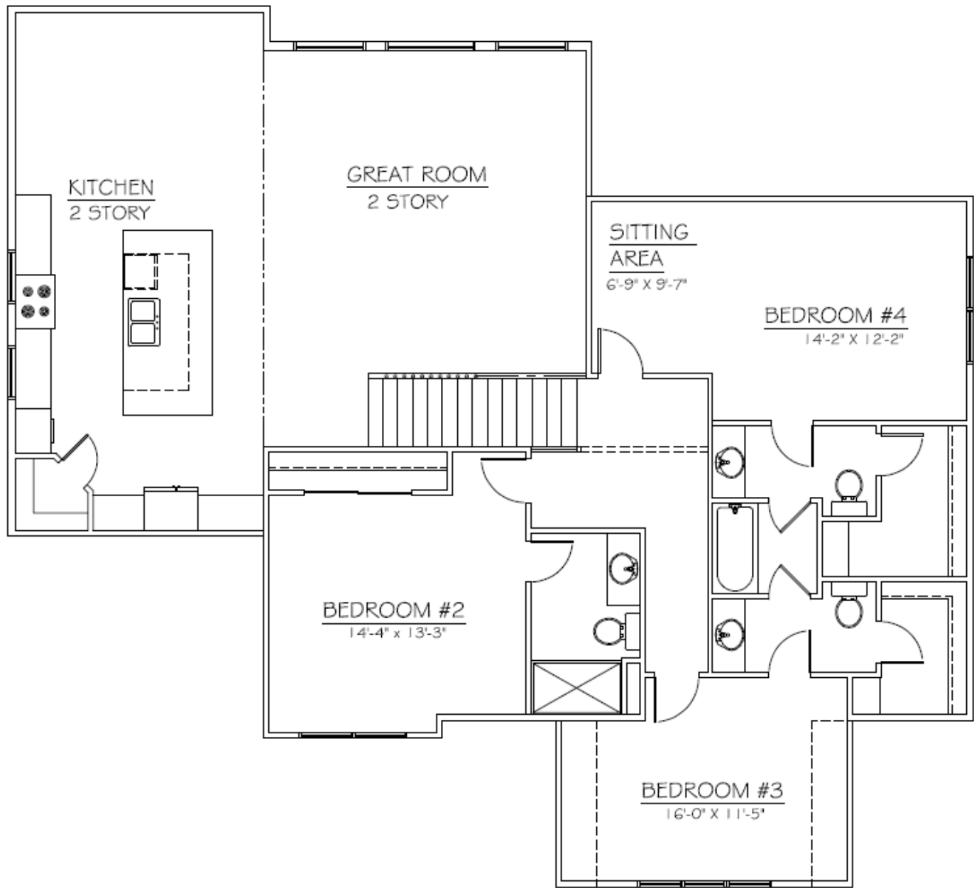
Second Floor Plan 1,077 Sq. Ft.
