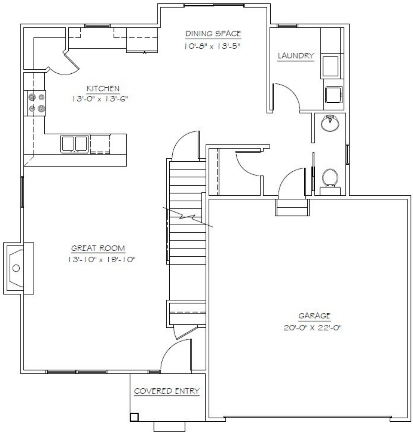
First Floor Plan 877 Sq Ft.
