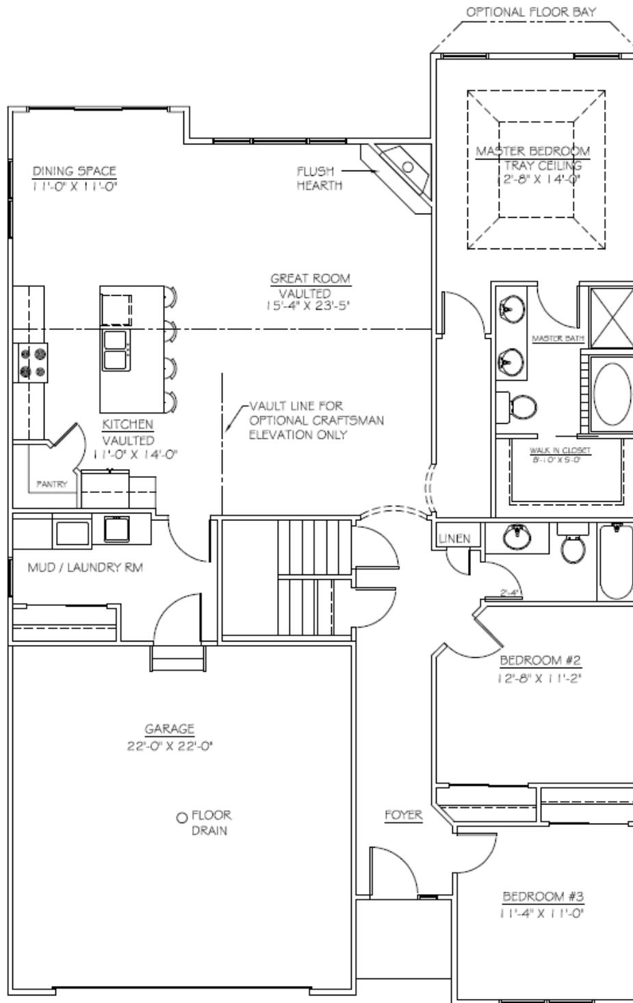
First Floor Plan 1,747 Sq. Ft.
