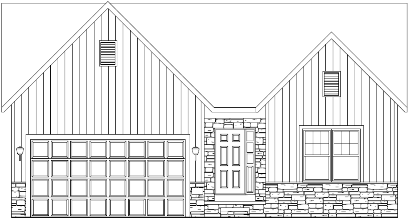
Modern Farm House Front Elevation
