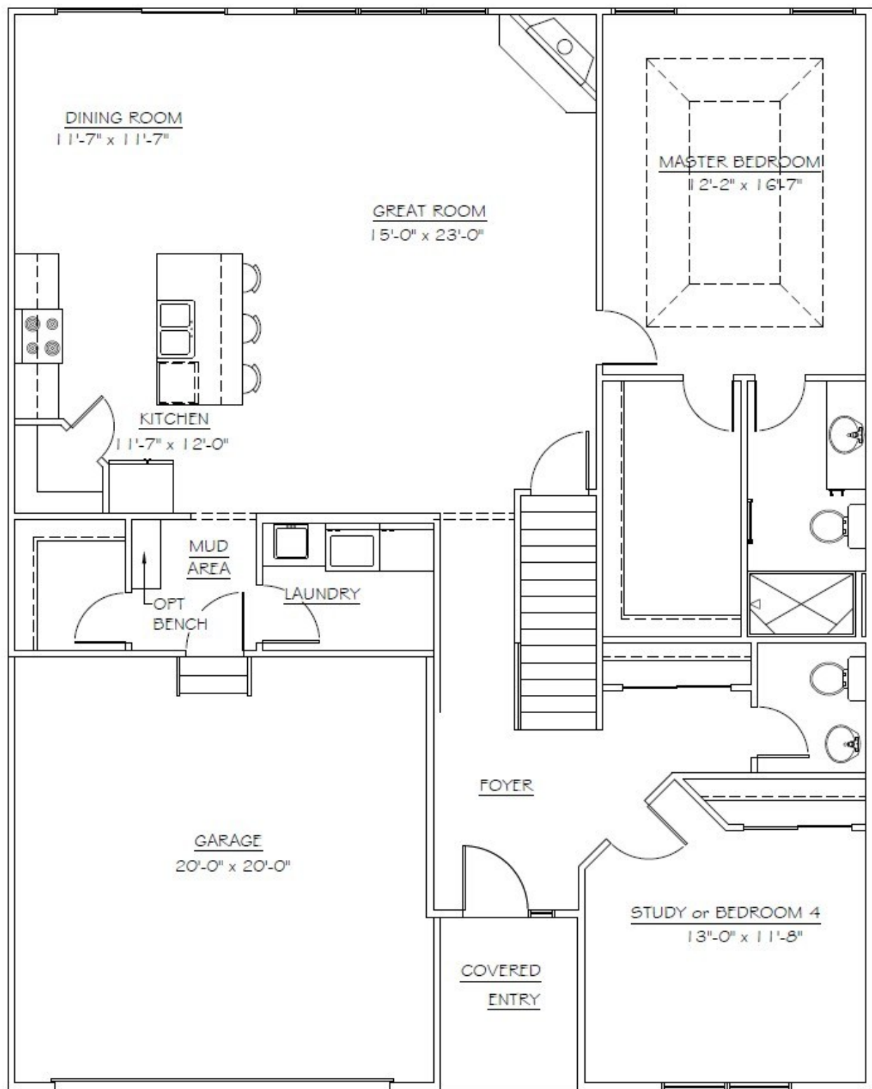
First Floor Plan 1,553 Sq. Ft.
