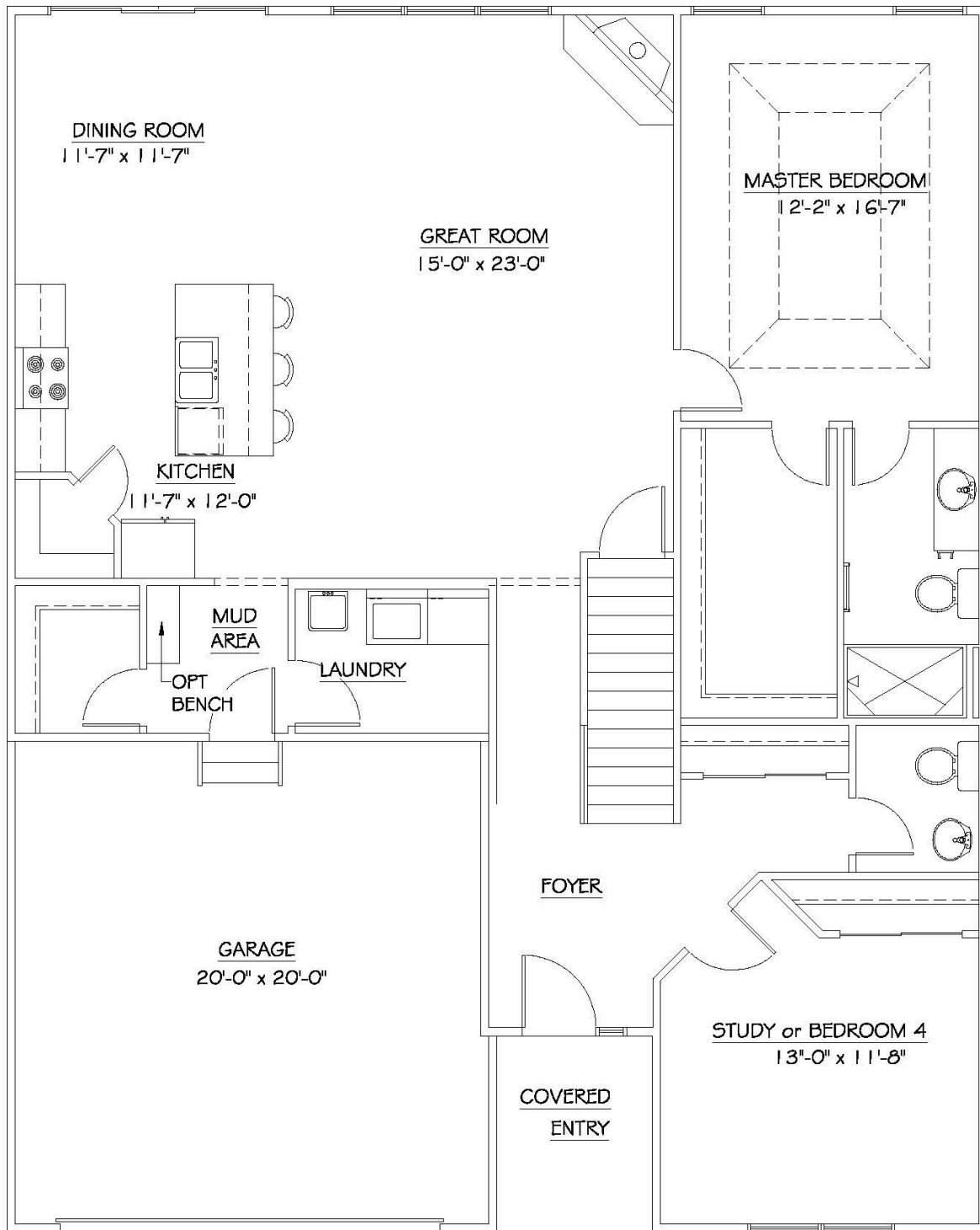
First Floor Plan 1,553 Sq. Ft.
