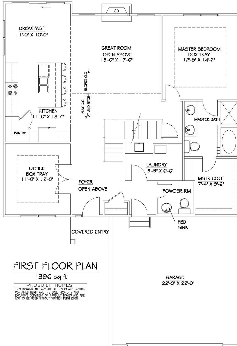
First Floor Plan 1,396 Sq. Ft.
