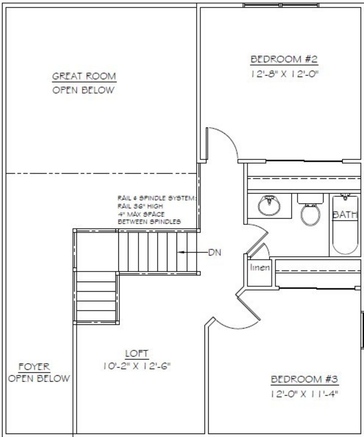
3 Bedroom Second Floor Plan Loft with 2 Story Foyer 581 Sq. Ft.
