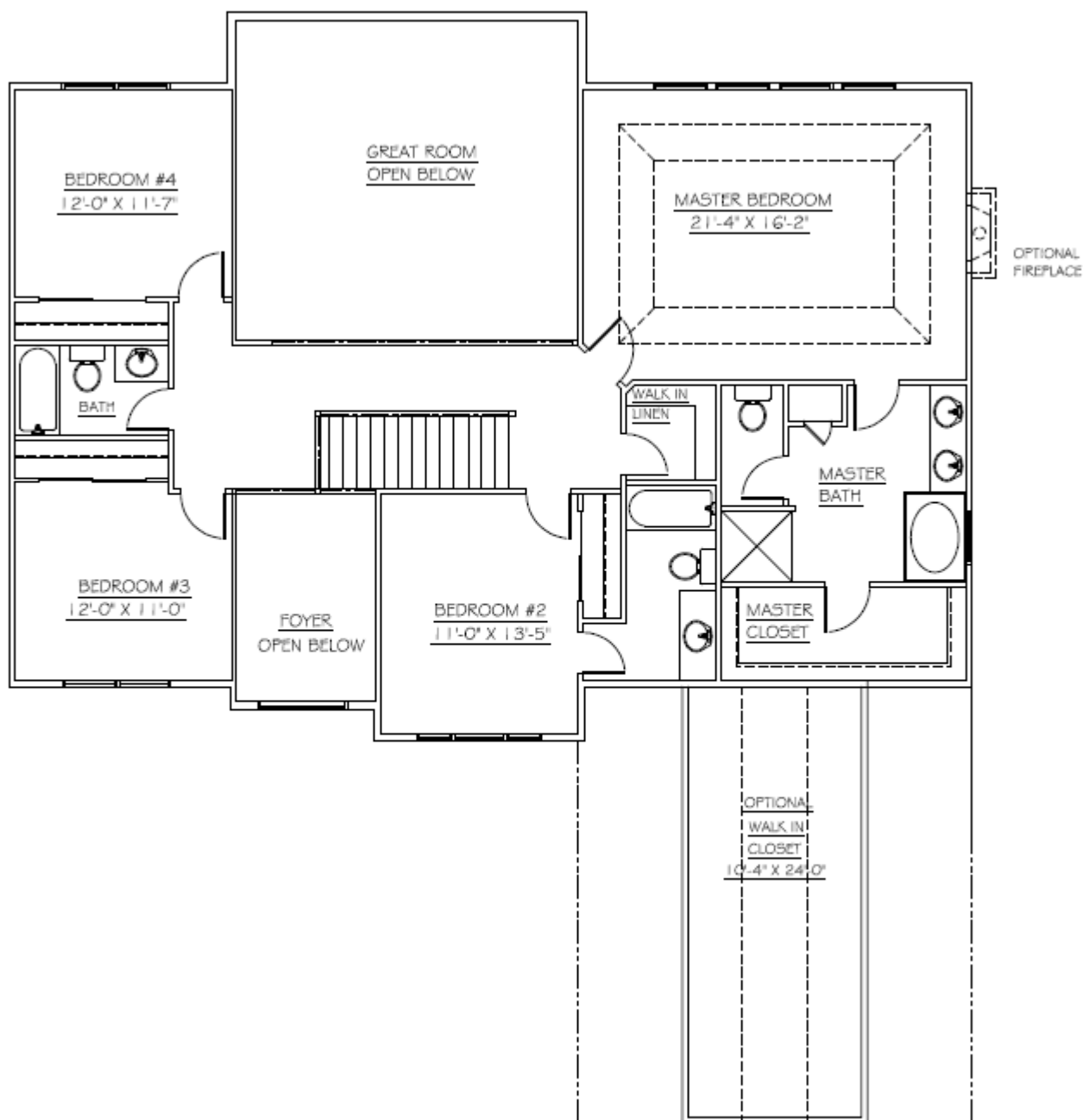
Second Floor Plan 1,443 Sq Ft.
