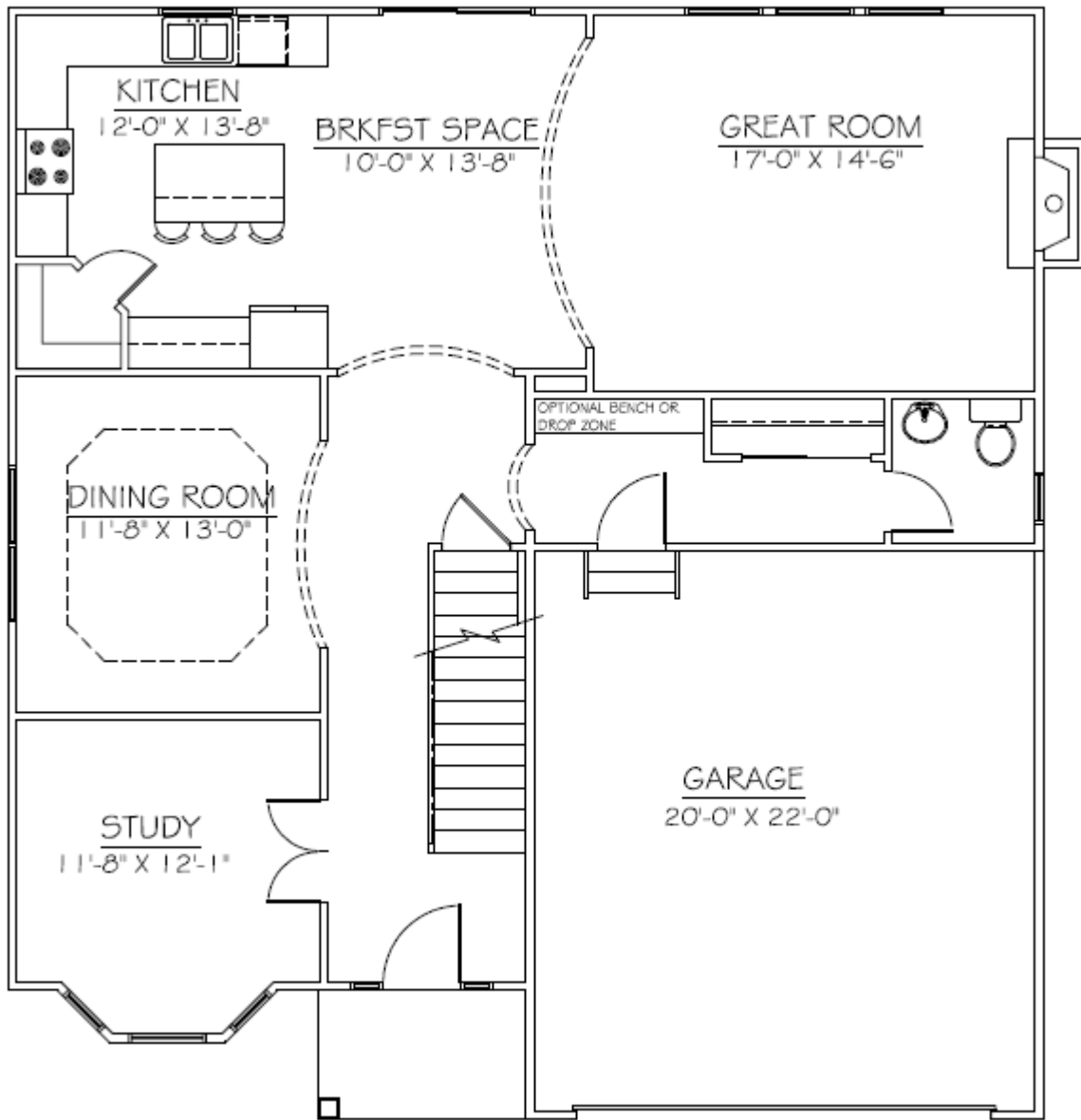
First Floor Plan 1,198 Sq. Ft.
