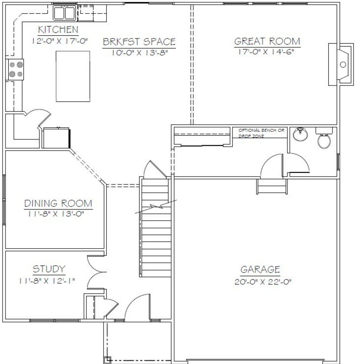
Standard First Floor Plan 1,185 Sq. Ft.
