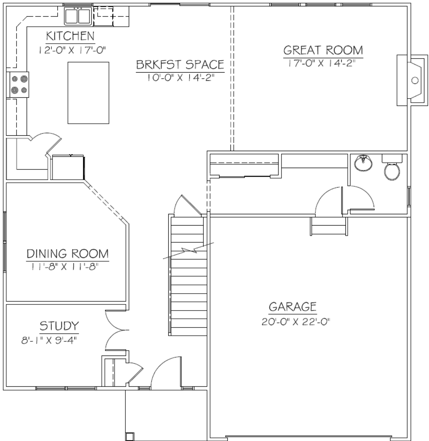
Standard First Floor Plan 1,198 Sq. Ft.
