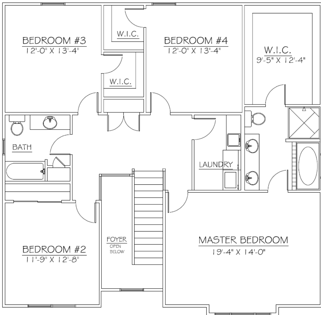
Second Floor Plan 1,404 Sq Ft.
