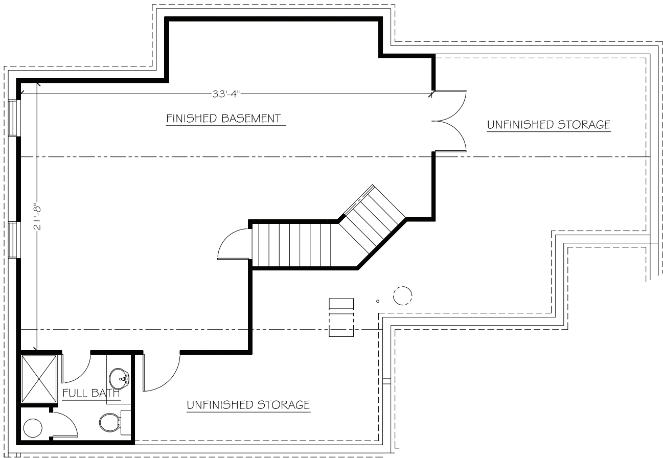
Basement Finish Plan 755 Sq. Ft.
