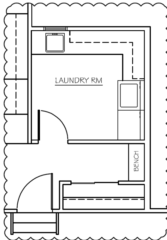
Optional Garage Entry / Laundry Room
