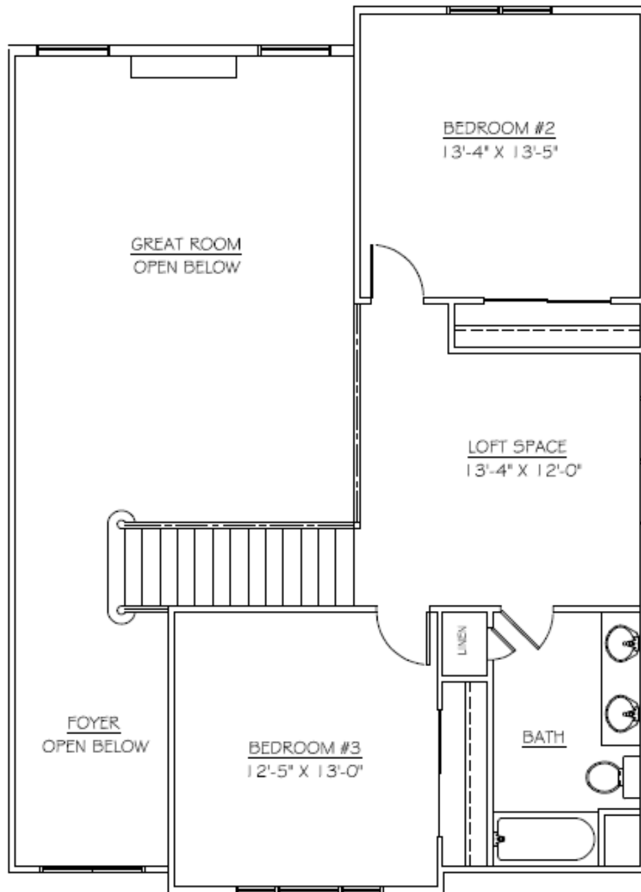
Optional Second Floor Plan #4 709 Sq. Ft.
