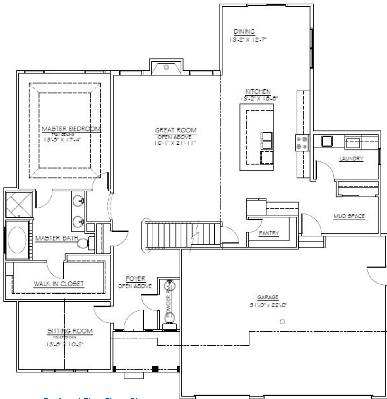
Optional First Floor Plan Optional Elevation 6 Only 2,096 Sq. Ft.
