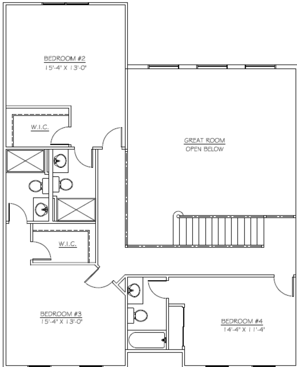
Second Floor Plan 1,104 Sq. Ft.
