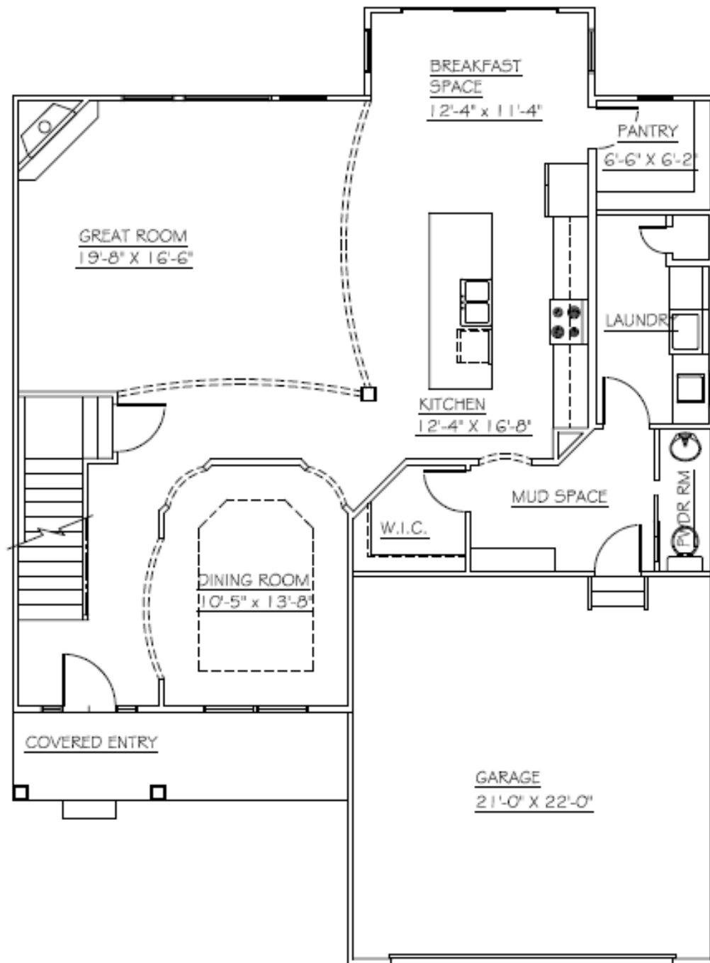
First Floor Plan 1,306 Sq. Ft.
