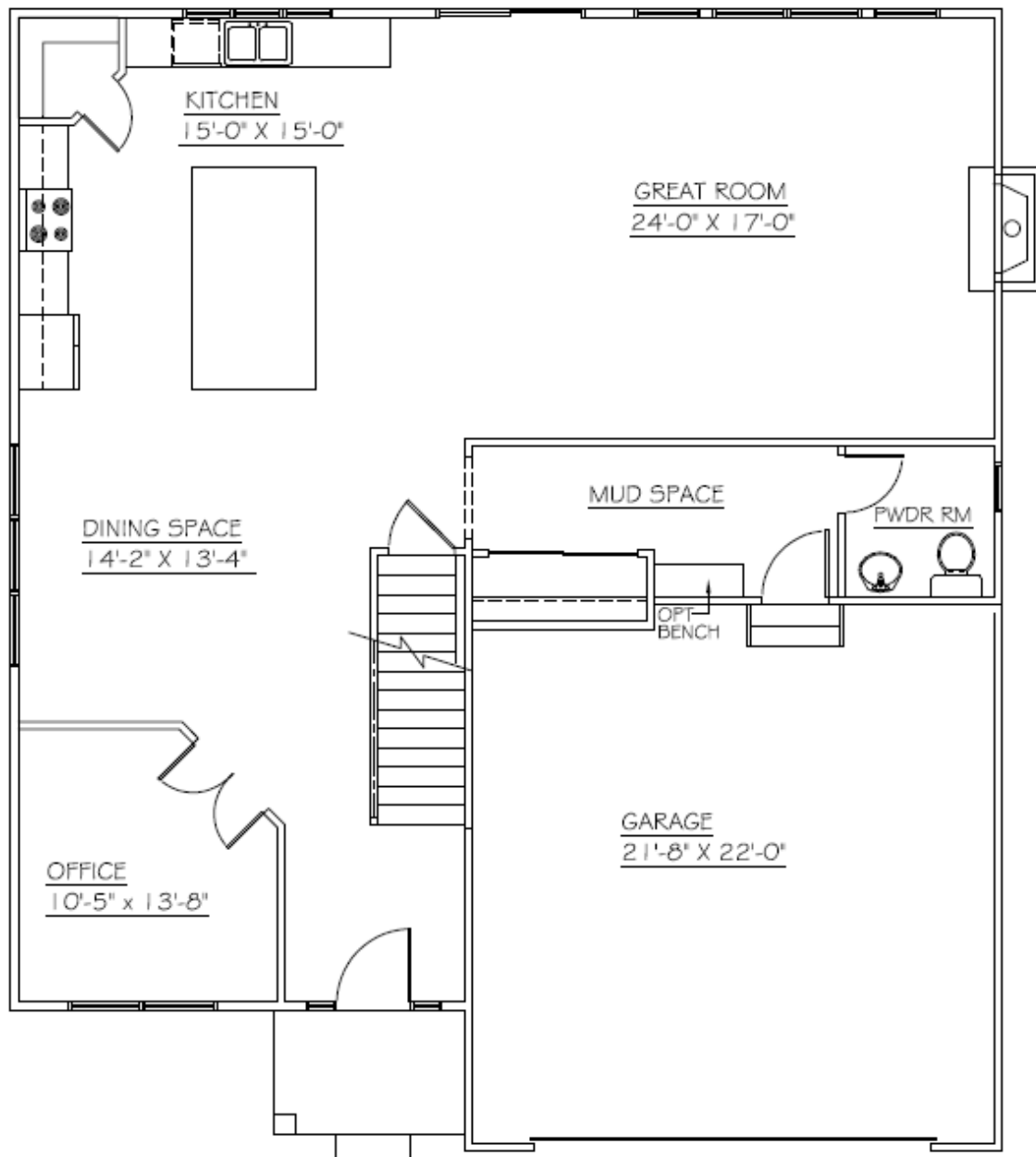
First Floor Plan 1272 Sq. Ft.
