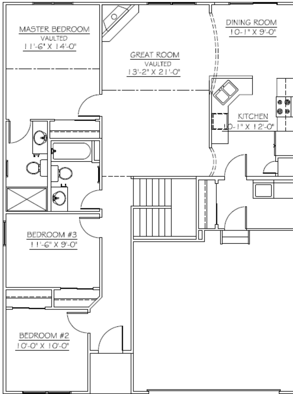
First Floor Plan—3 Bedroom with Basement 1,301 Sq. Ft.
