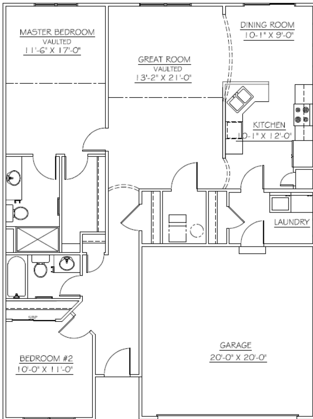
First Floor Plan— 2 Bedroom Slab 1,301 Sq. Ft.
