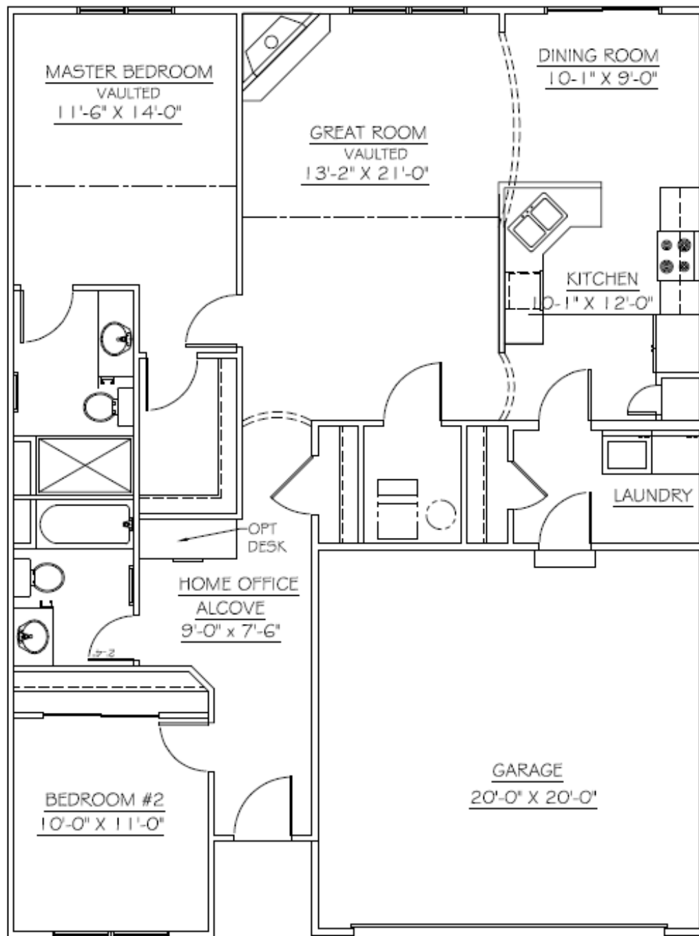
First Floor Plan— 2 Bedroom with Home Office Alcove Slab 1,301 Sq. Ft.
